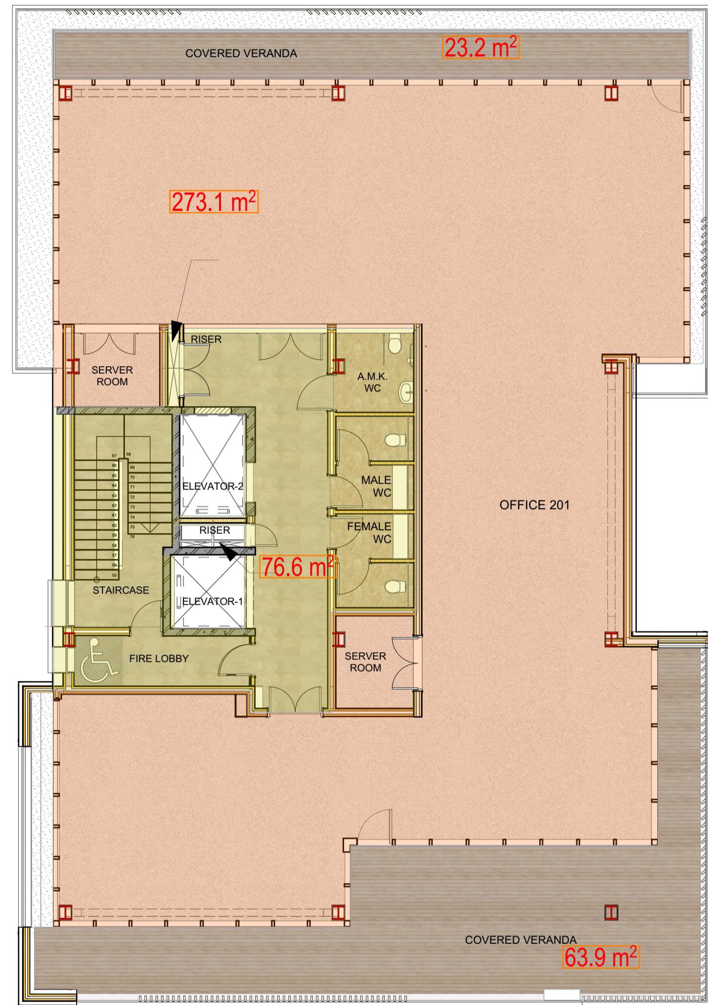
3. | 2ND FLOOR PLAN 1:100
