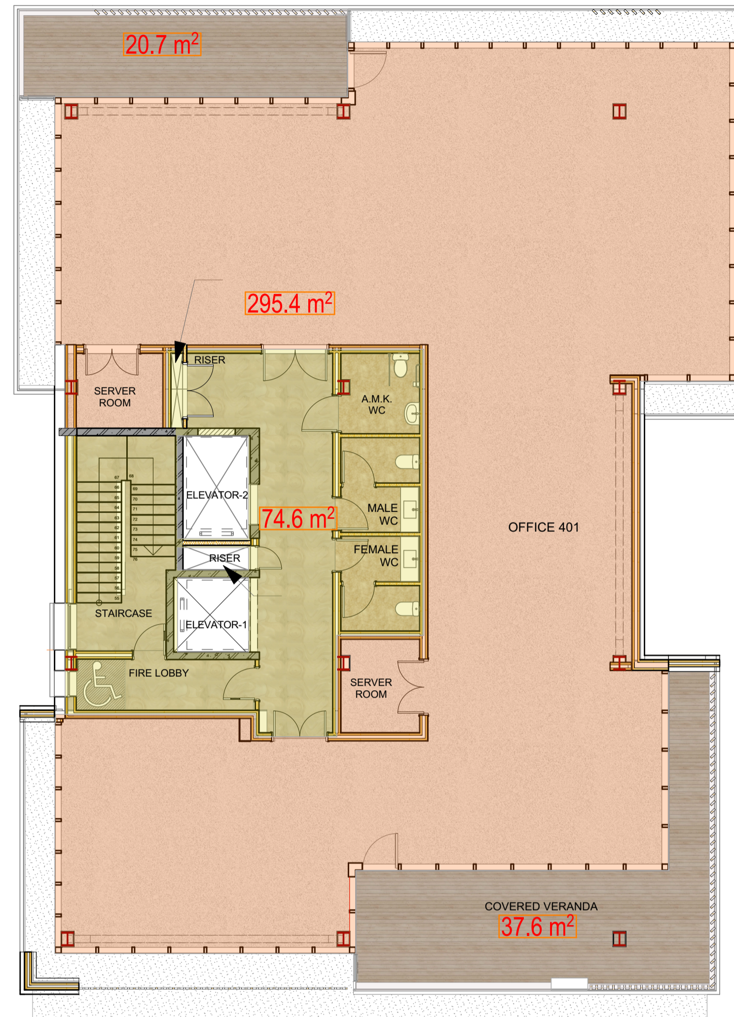
5. 4TH FLOOR PLAN 1:100
