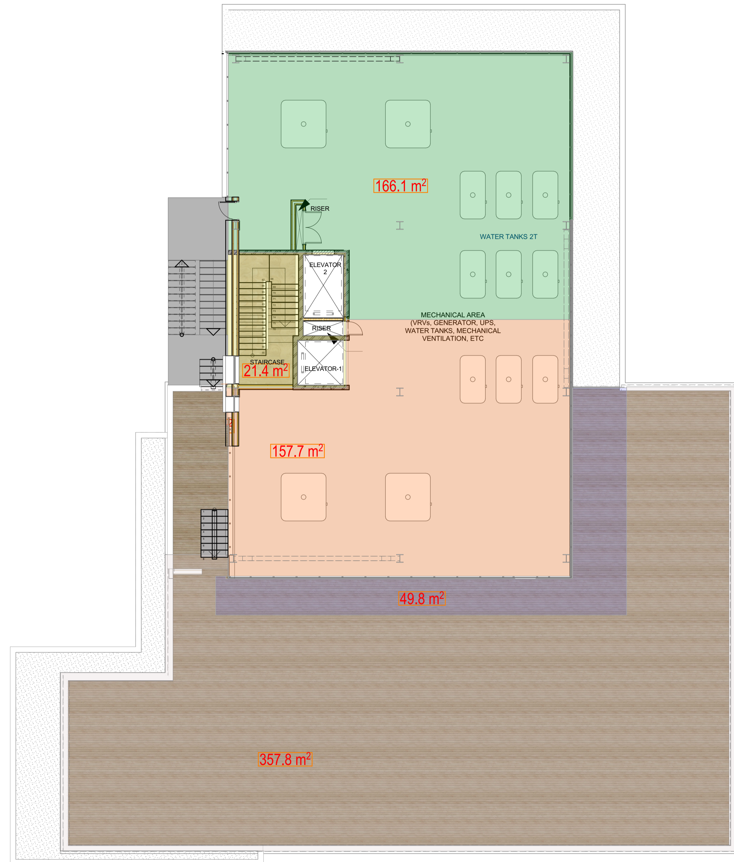
1. MEZZANINE/MECHANICAL FLOOR PLAN 1:100
