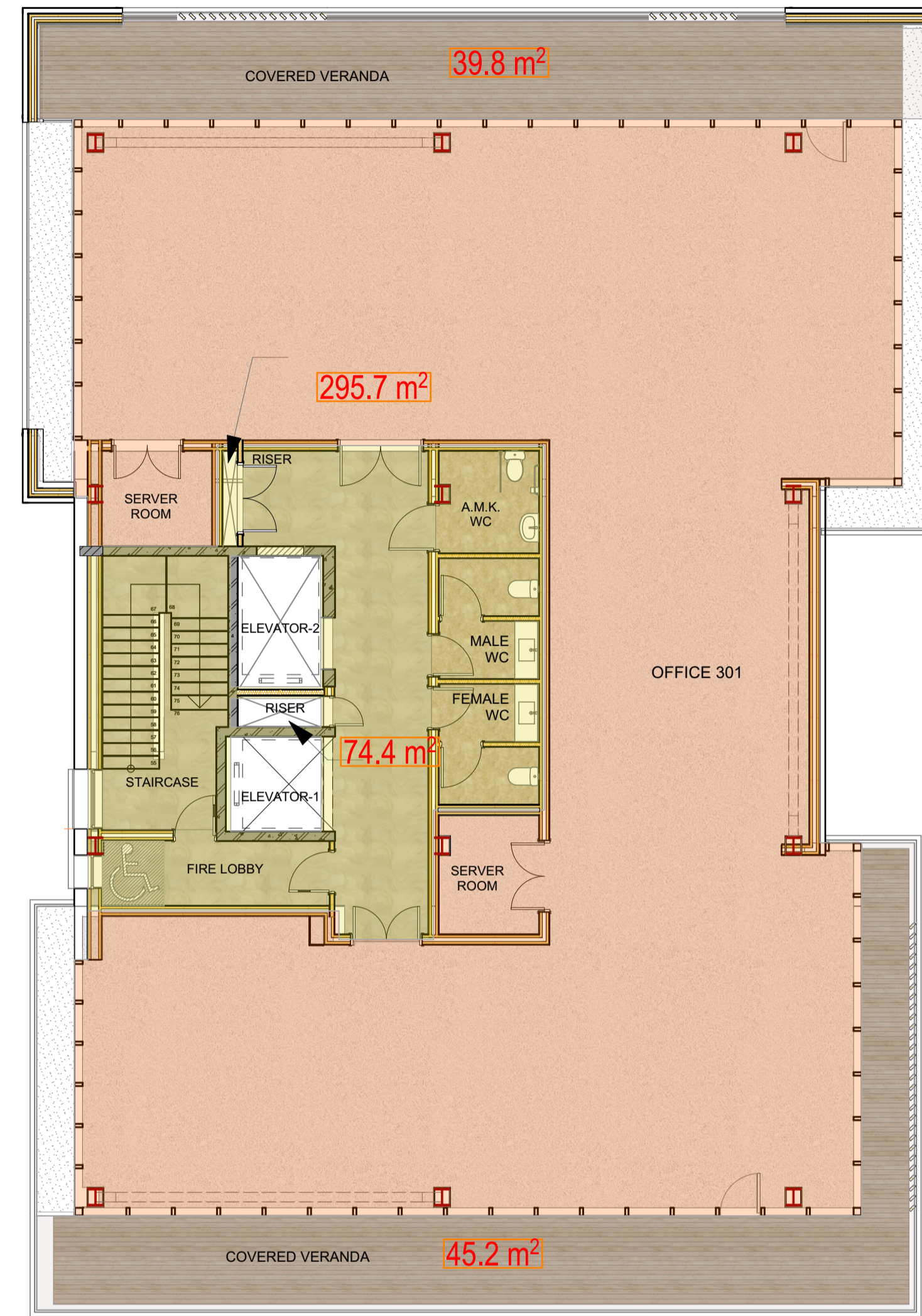
4. | 3RD FLOOR PLAN 1:100
